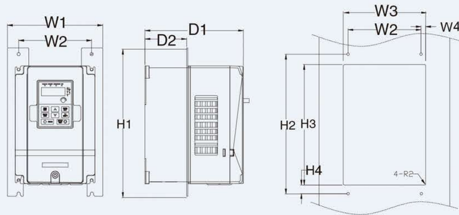
Flange mounting for the 4-200kW models
