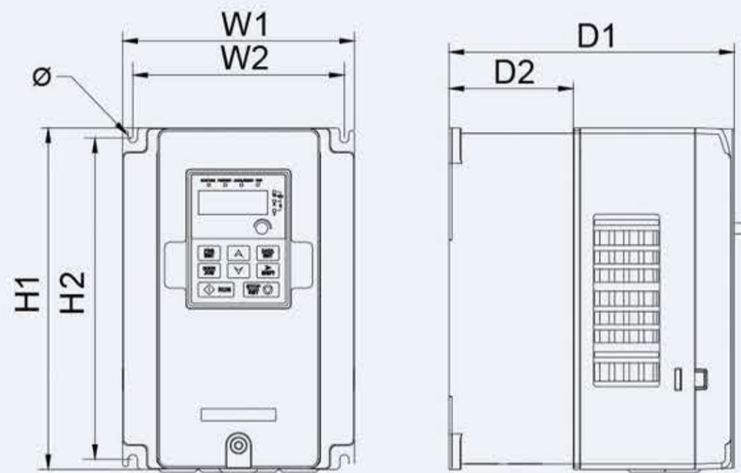
Wall mounting for the 4~200kW models
