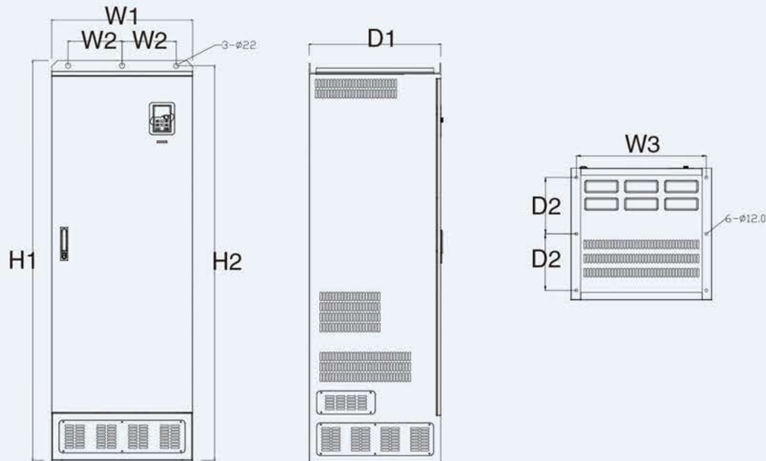
Floor mounting for the 355-500kW models
