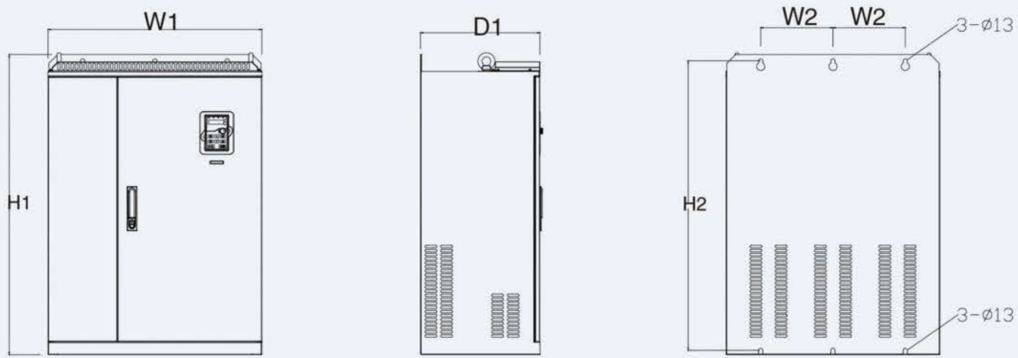
Flange mounting for the 4-200kW models
