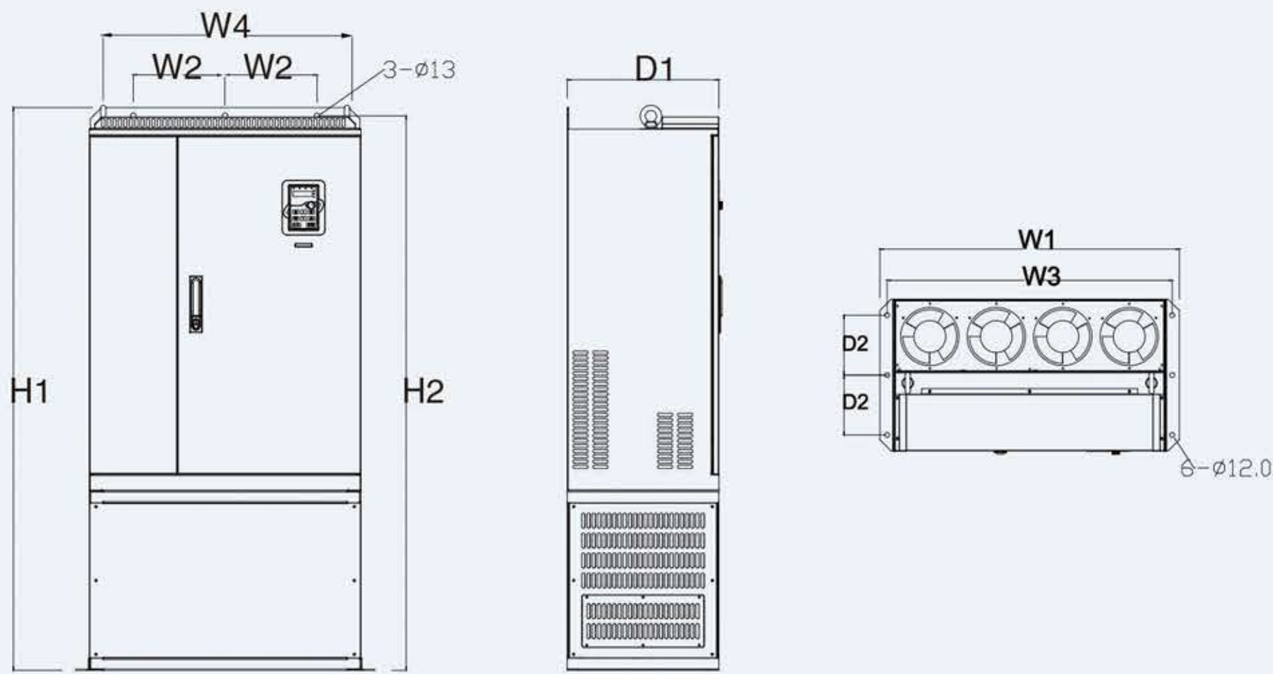
Floor mounting for the 220-315kW models
