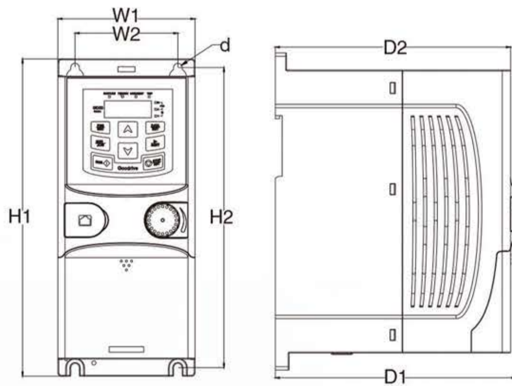
Wall mounting for models below 2.2kW
