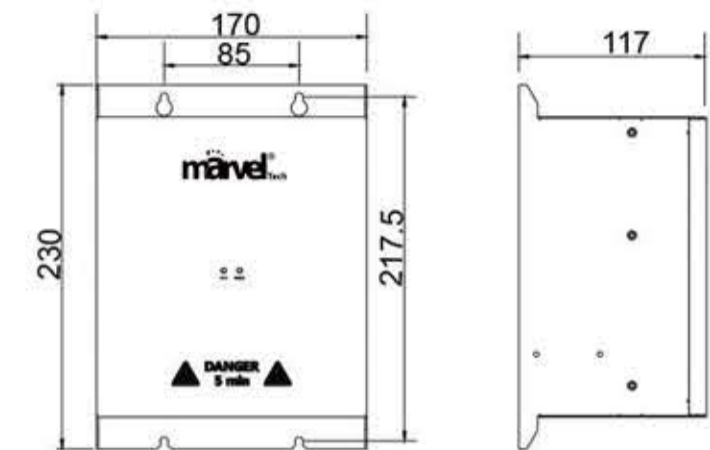
Installation dimension
