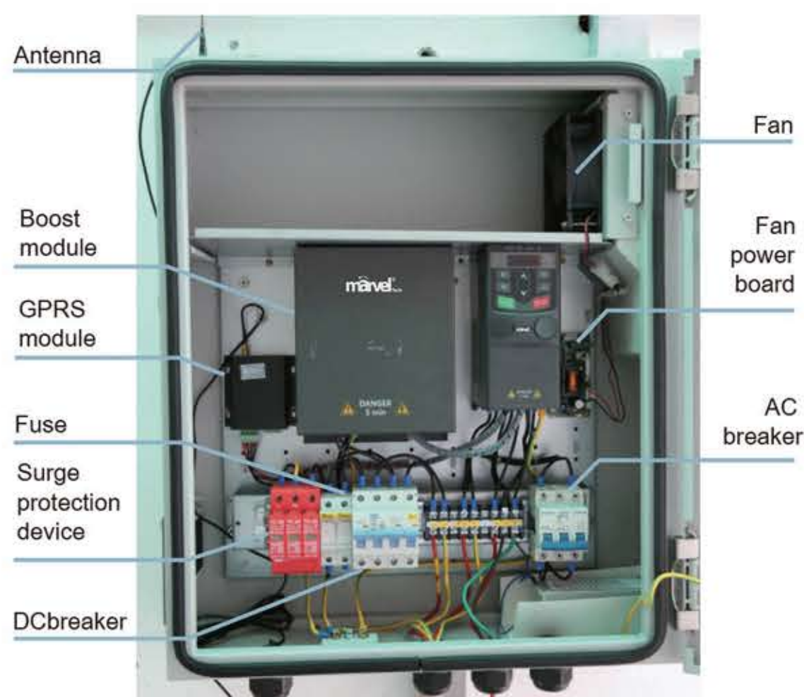
Internal structure of GD100-2R2G-S25-PV-AS
