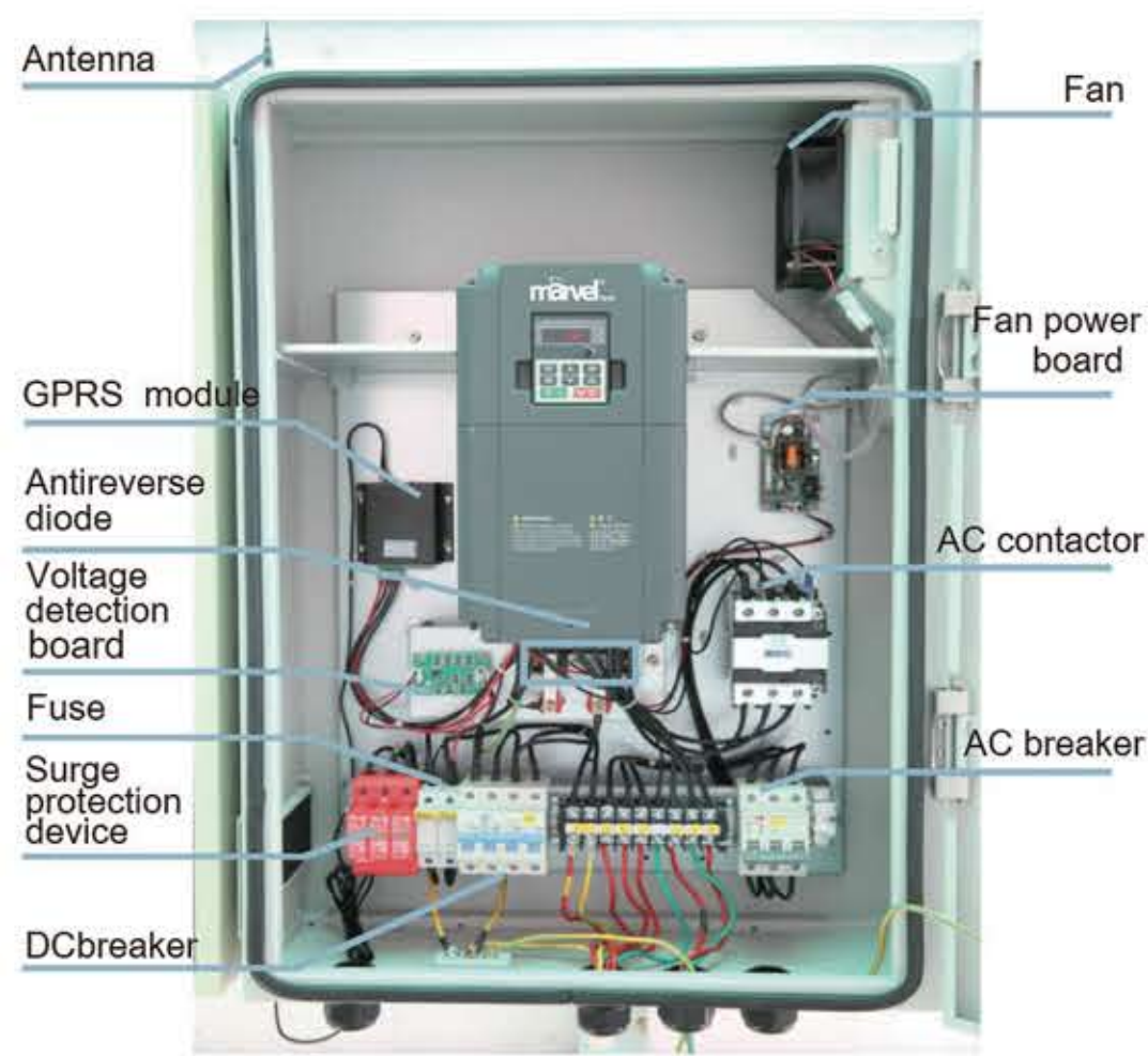
Internal structure of GD100-015G-45-PV-AS
