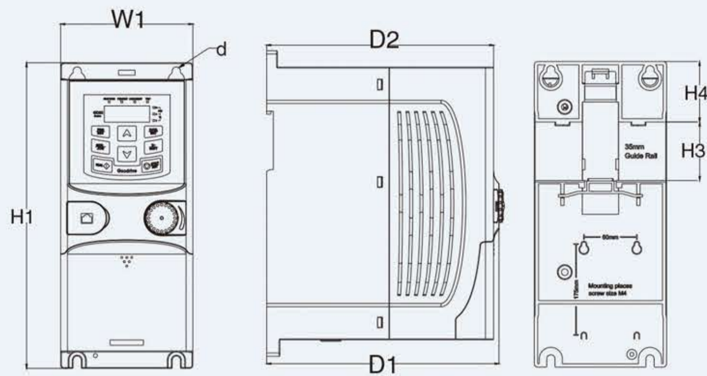
Rail mounting for the models below 2.2kW
